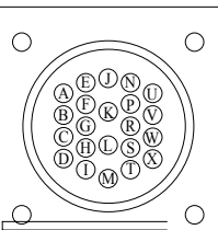
AMPHENOL MS3102E28-11P Cable-End Connector Rear View
